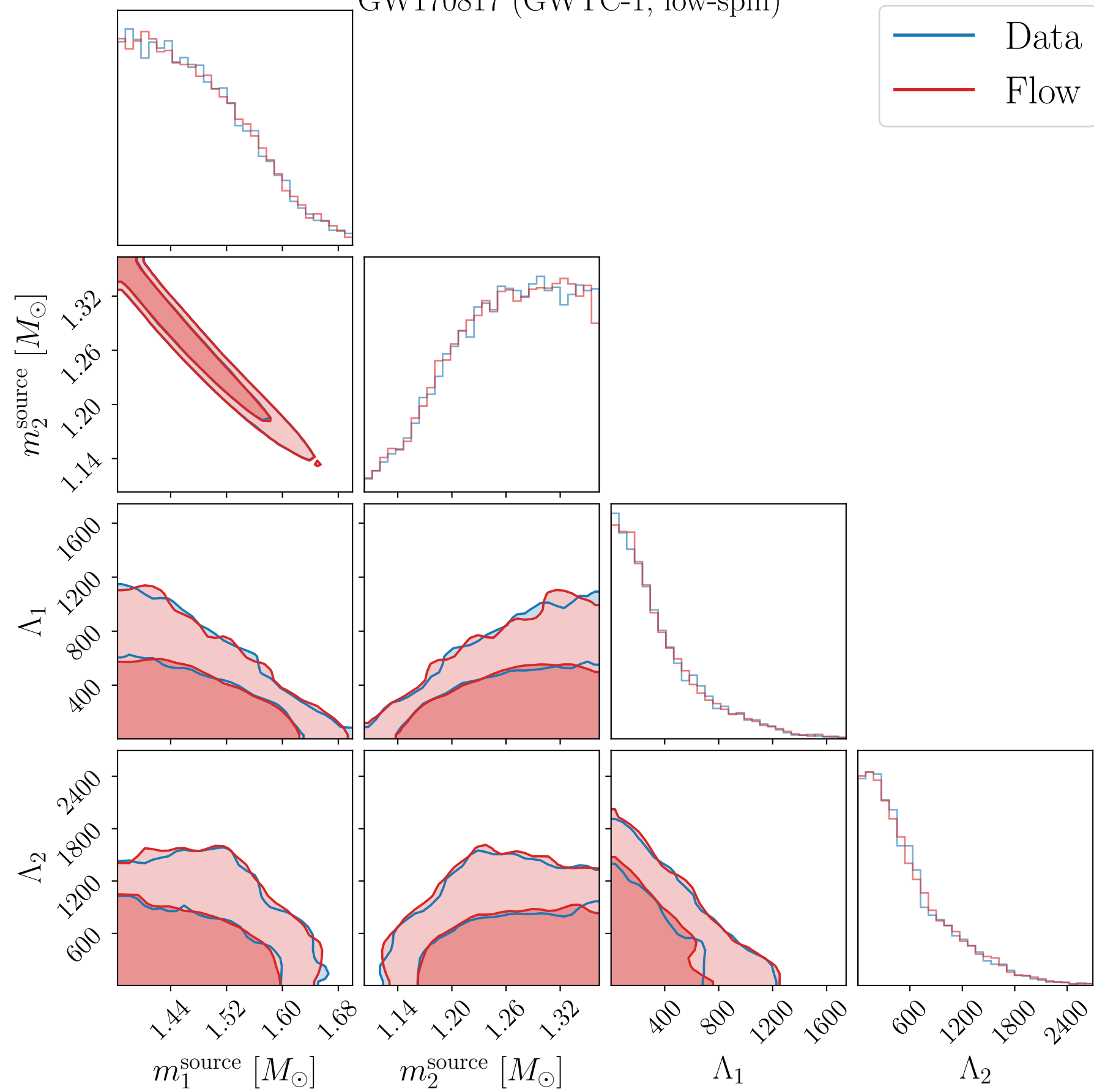
GW170817 (GWTC-1, low-spin)
